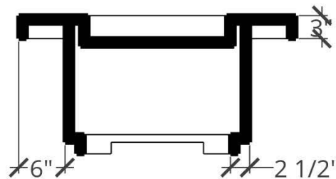
SIDE ELEVATION
