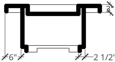
SIDE ELEVATION
